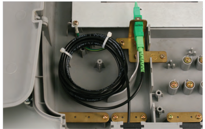
ONT open with W7 cable installed and tight coil of tight buffer drop shown.
